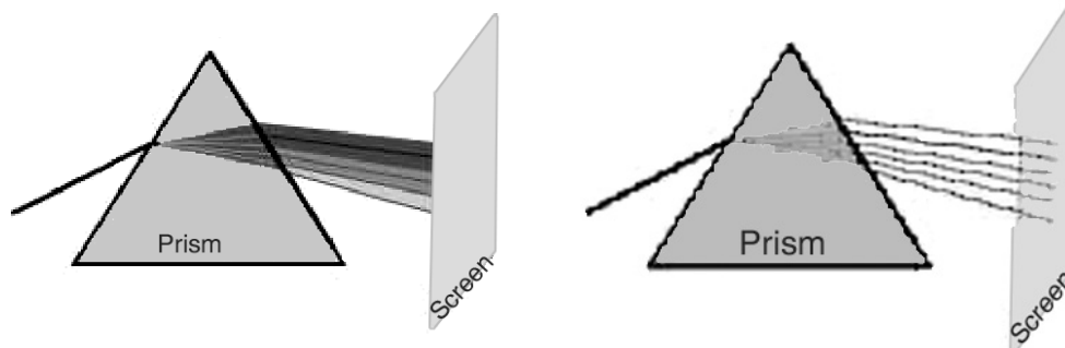
Fig. 2.8: a) a Continuous spectrum
