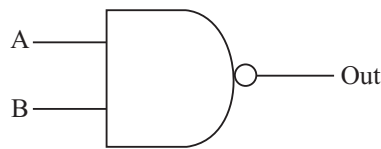
Fig. 2.6: NAND Gate representation
