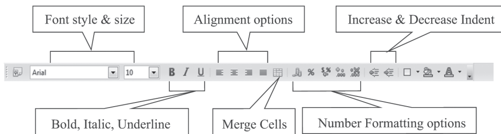
Fig. 9.22: Formatting Toolbar
