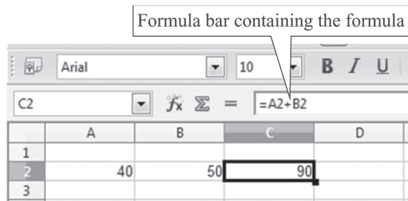
Fig. 9.7: Entering Formula
