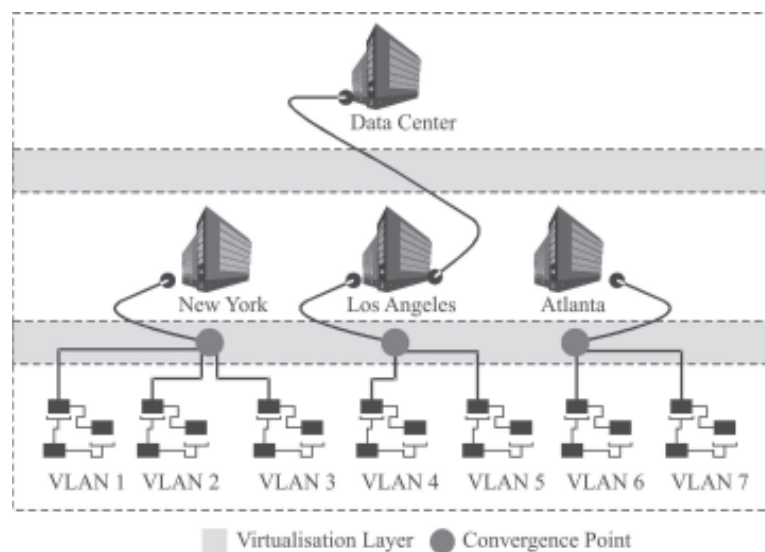
Fig. 26.2: Network Virtualization
