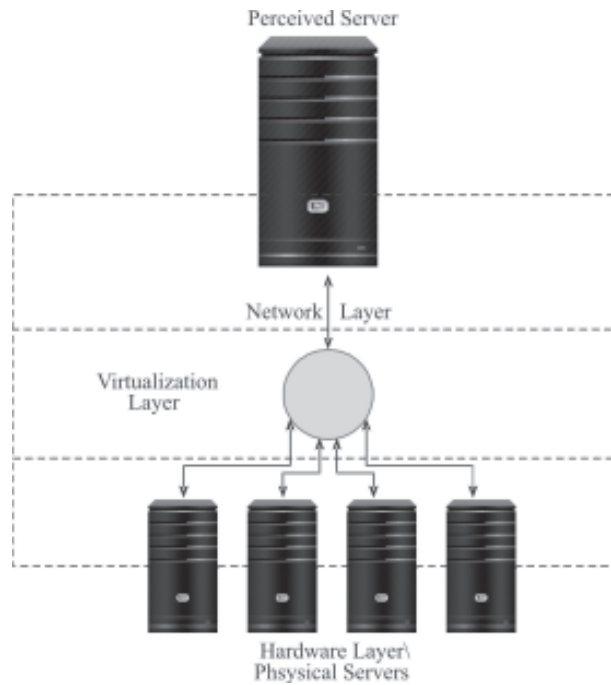
Fig. 26.1: Server Virtualization
