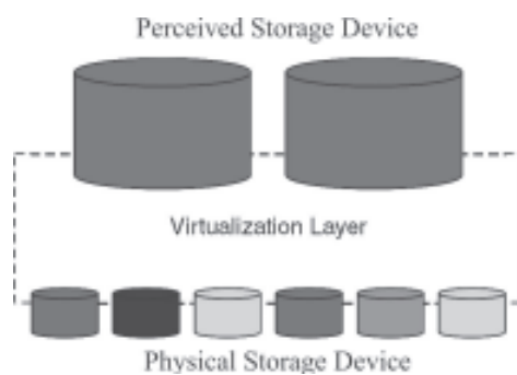
Fig. 26.3: Storage Virtualization
